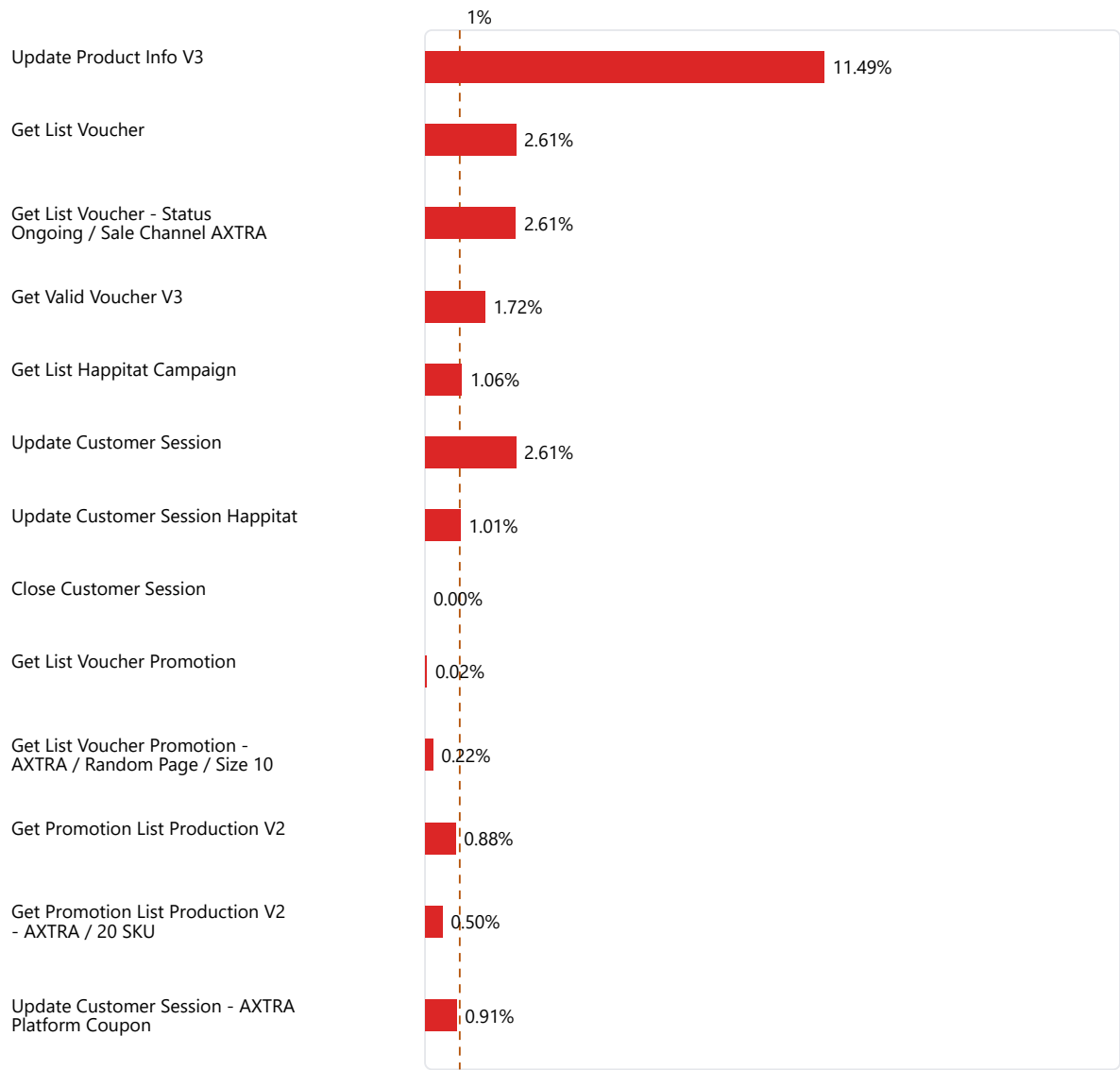
Maximum Error Rate by API — Main comparison range
