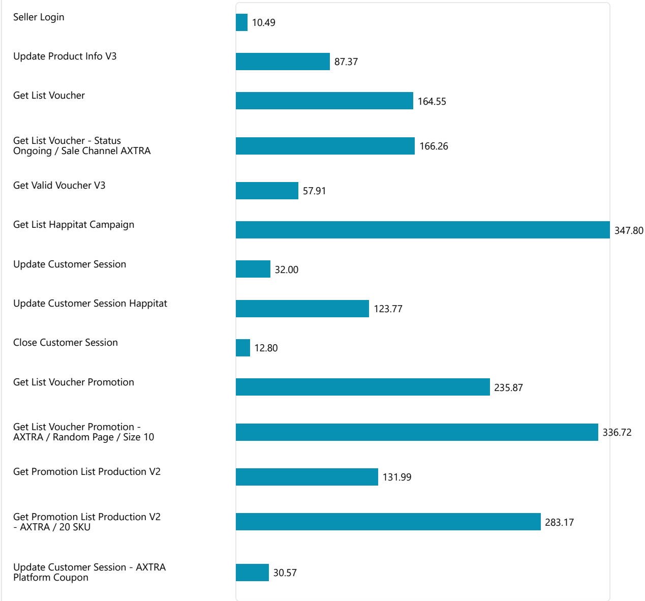
TPS by API at representative load (informational)
