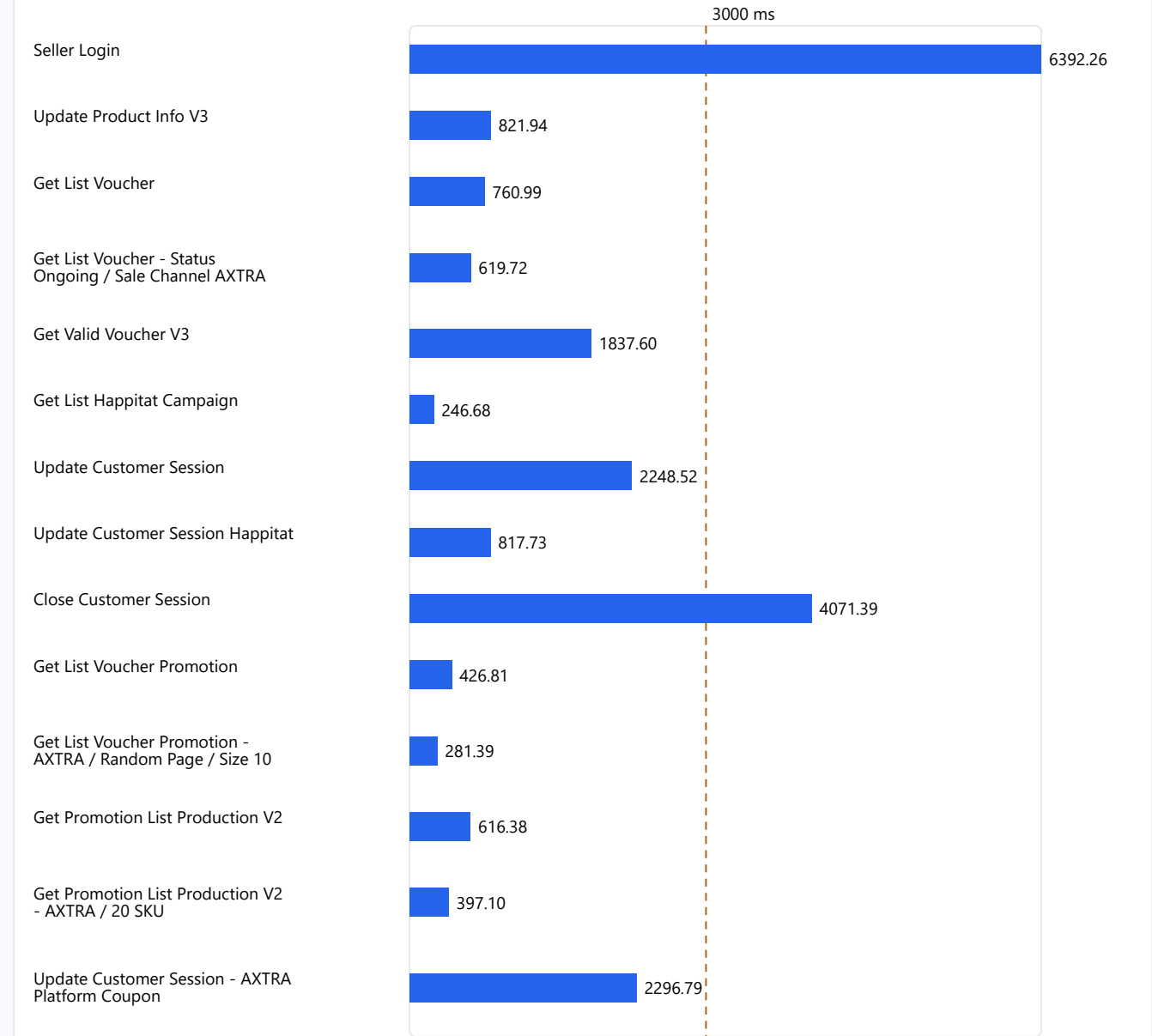
P95 by API at representative load
